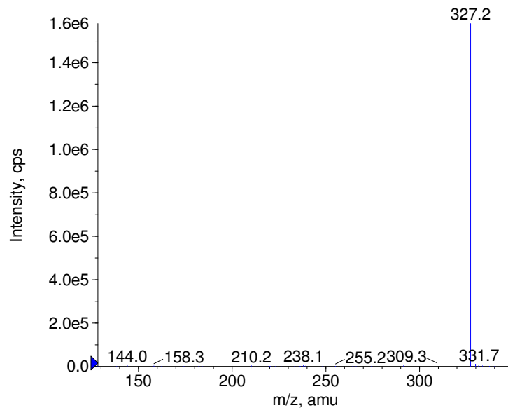
+ Ajmaline Prec(327.0) CE(50.0) RT(0.7)
