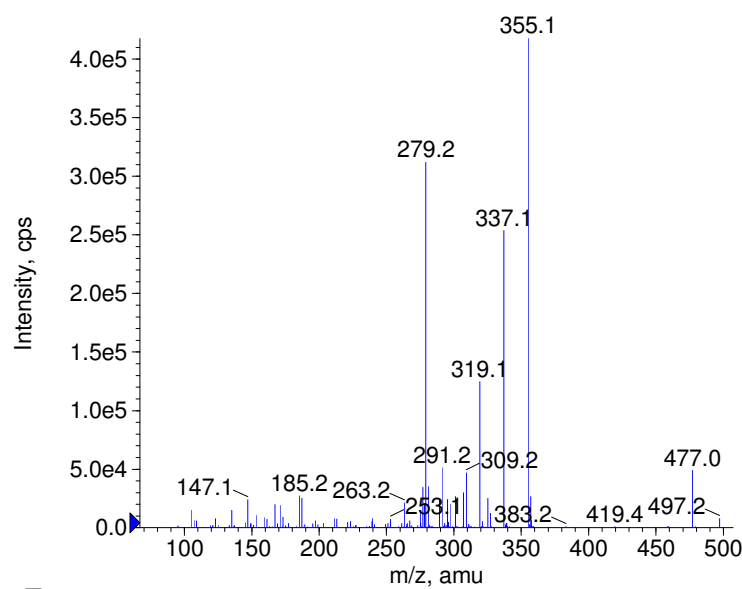
+ Betamethasone-17-benzoate Prec(497.0) CE(50.0) RT(1.5)
