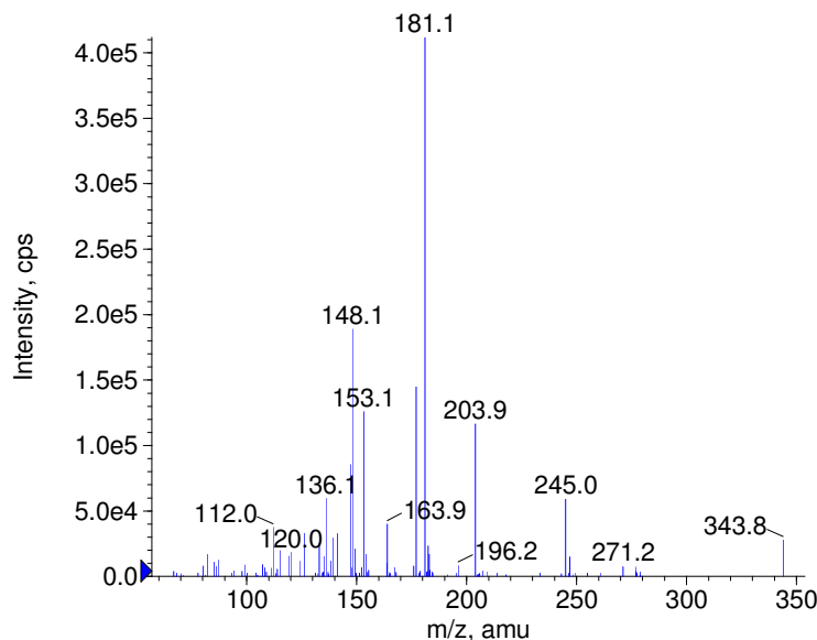
■ + Cefazedone Prec(548.0) CE(50.0) RT(0.9)
