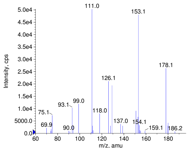
+ Chlorazaniil Prec(222.0) CE(50.0) RT(0.9)
