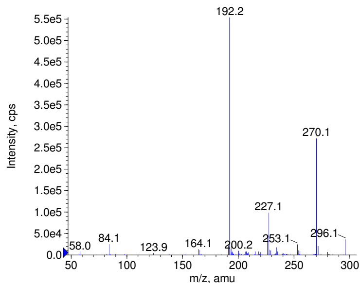
+ Clozapine Prec(327.0) CE(50.0) RT(0.8)
