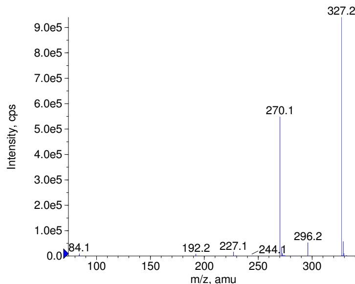
+ Clozapine Prec(327.0) CE(50.0) RT(0.8)
