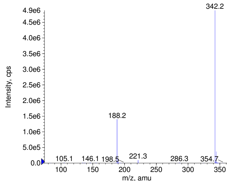
+ D5-Fentanyl Prec(342.0) CE(50.0) RT(0.8)
