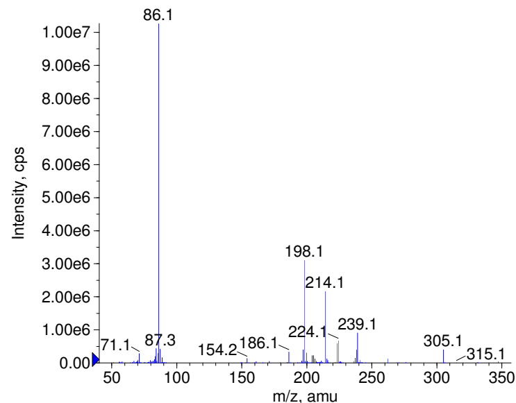
+ Dimetotiazine Prec(392.0) CE(50.0) RT(0.9)
