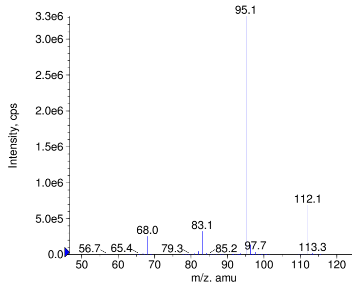
+ Histamine Prec(112.0) CE(50.0) RT(1.2)
