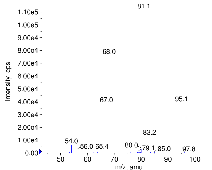
+ Histamine Prec(112.0) CE(50.0) RT(1.2)
