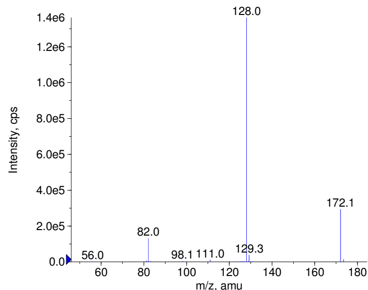
+ Metronidazole Prec(172.0) CE(50.0) RT(0.7)
