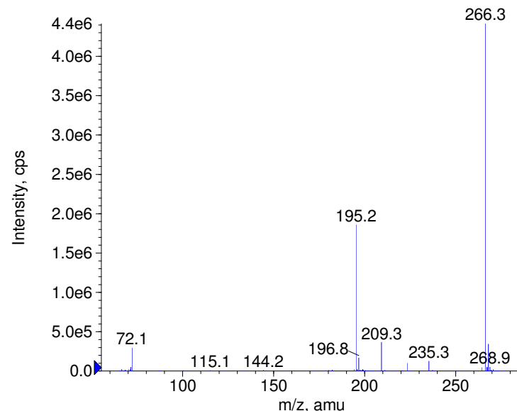
+ Mirtazapine Prec(266.0) CE(50.0) RT(0.7)
