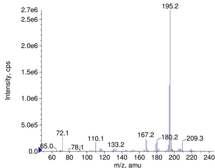
+ Mirtazapine Prec(266.0) CE(50.0) RT(0.7)
