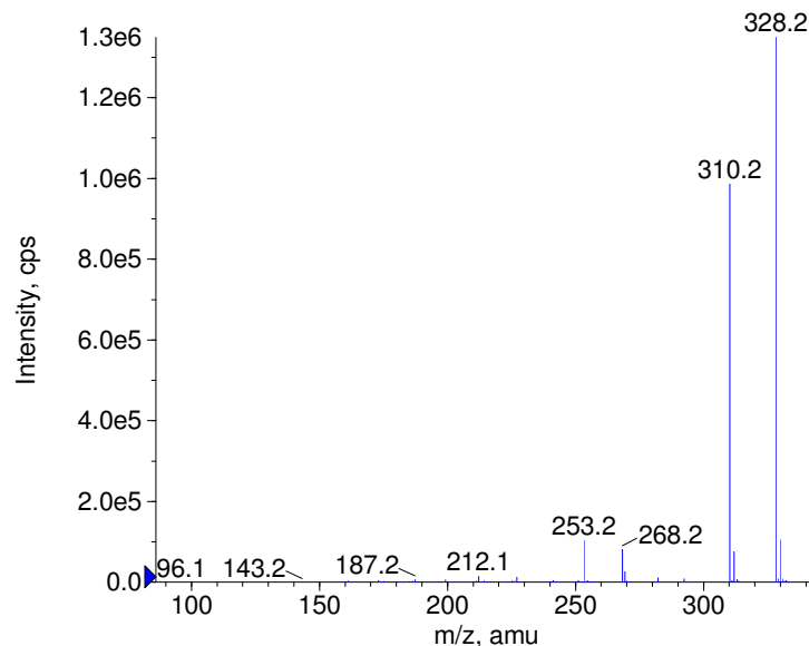
+ Naloxone Prec(328.0) CE(50.0) RT(0.7)
