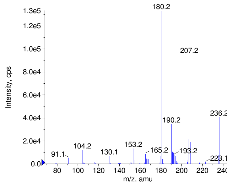
+ Nitrazepam Prec(282.0) CE(50.0) RT(0.9)
