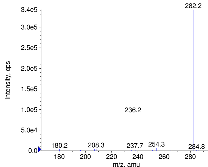
+ Nitrazepam Prec(282.0) CE(50.0) RT(0.9)
