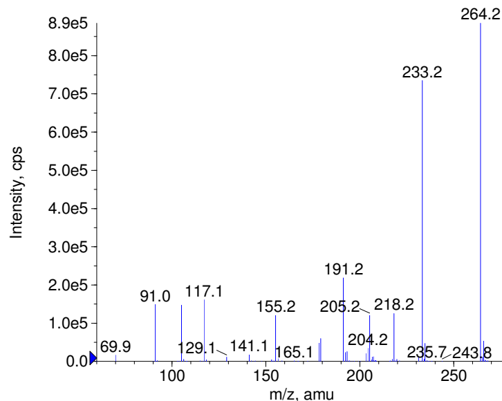
■ + Nortriptyline Prec(264.0) CE(50.0) RT(0.8)
