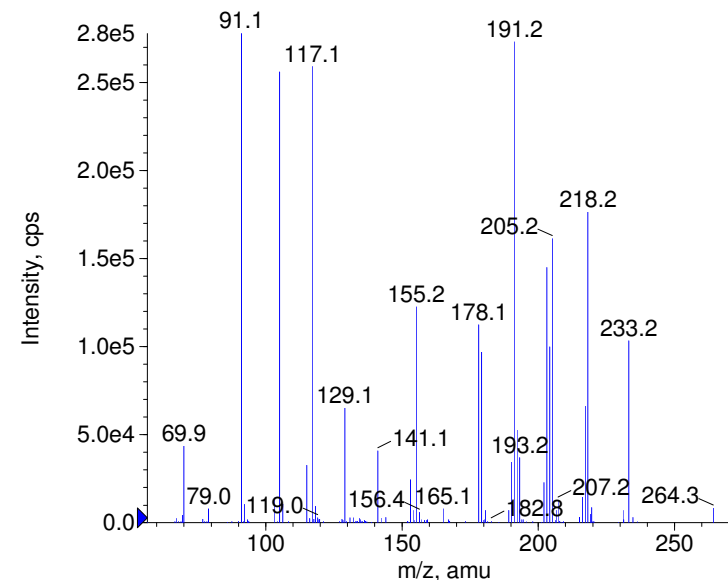
■ + Nortriptyline Prec(264.0) CE(35.0) RT(0.8)
