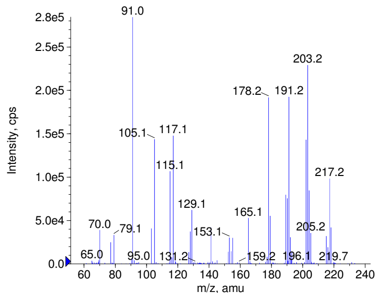
■ + Nortriptyline Prec(264.0) CE(50.0) RT(0.8)
