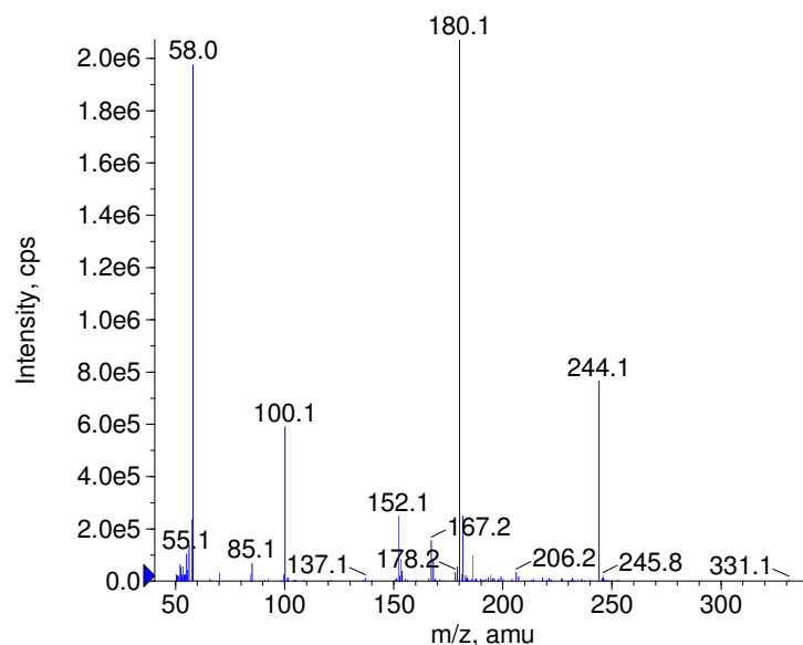
+ Oxomemazine Prec(331.0) CE(50.0) RT(0.8)
