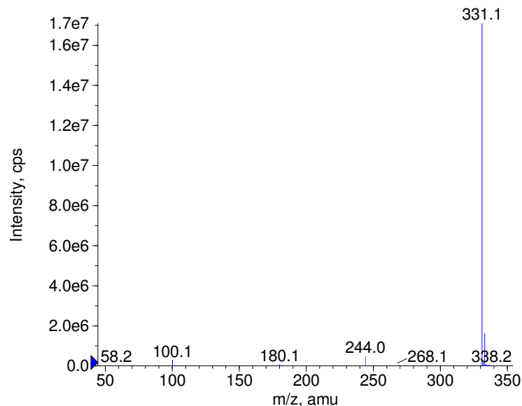
+ Oxomemazine Prec(331.0) CE(50.0) RT(0.8)
