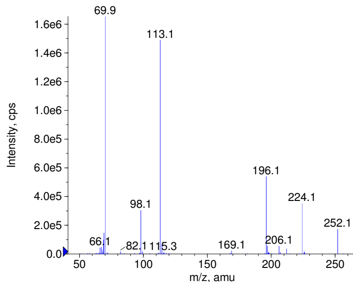
+ Pirenzepine Prec(352.0) CE(50.0) RT(0.8)
