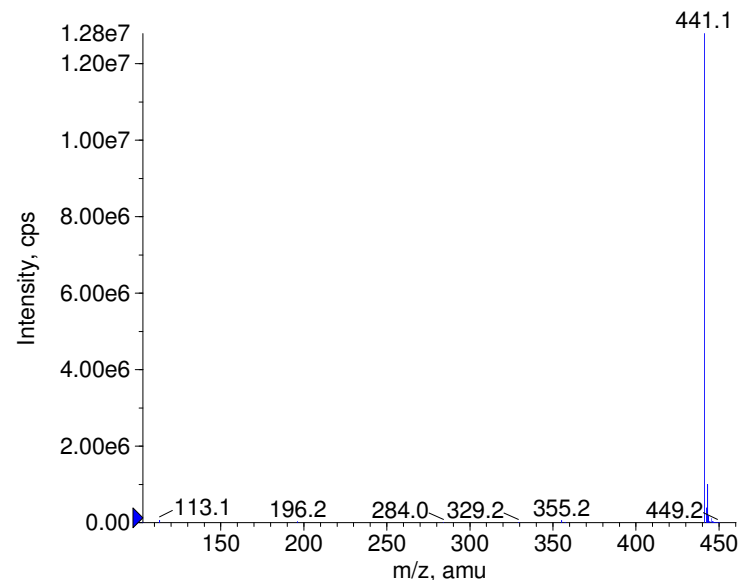
+ Sertindole Prec(441.0) CE(50.0) RT(0.8)
