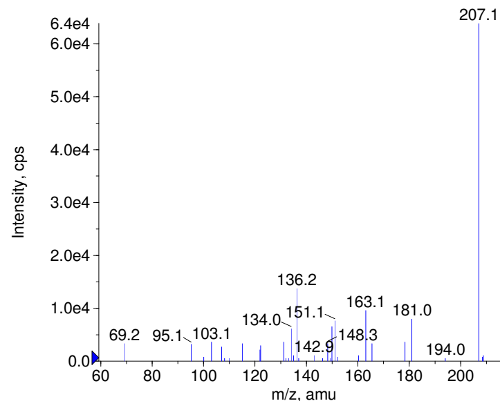
+ Theodrenaline Prec(376.0) CE(50.0) RT(0.7)
