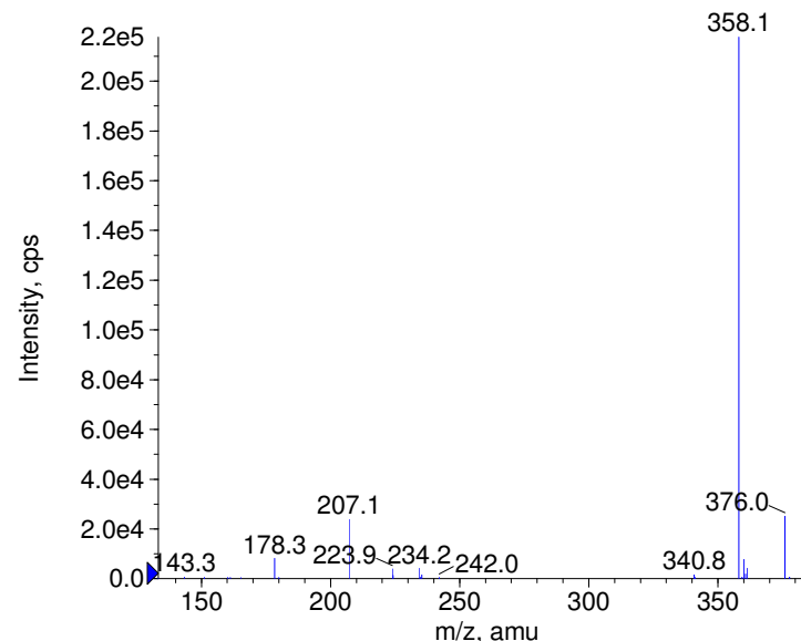
+ Theodrenaline Prec(376.0) CE(50.0) RT(0.7)
