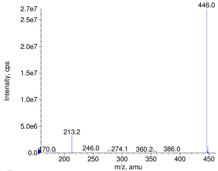
+ Thiopropazate Prec(446.0) CE(50.0) RT(0.9)
