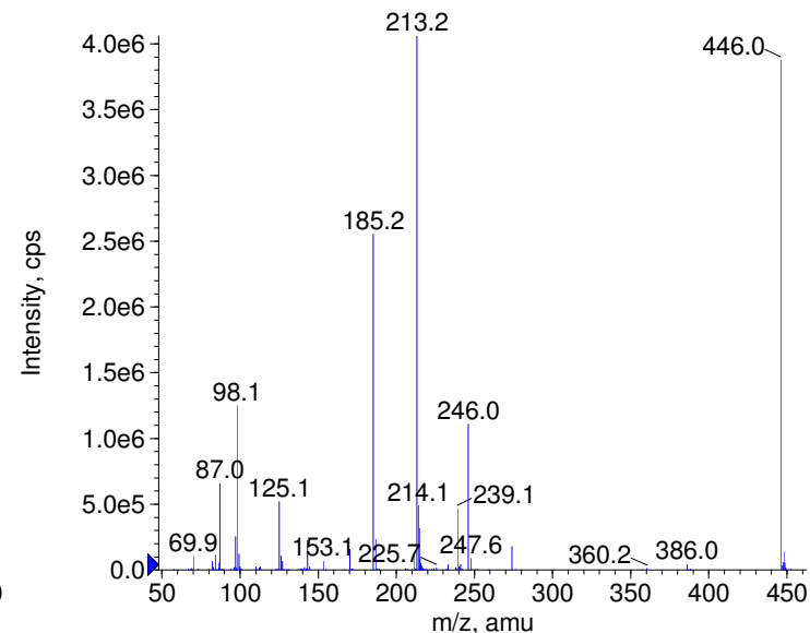
+ Thiopropazate Prec(446.0) CE(99.0) RT(0.9)
