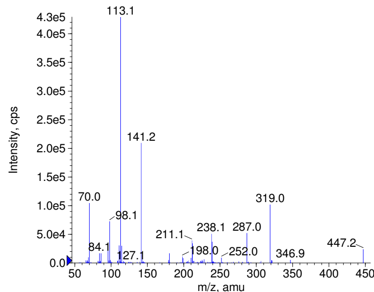
+ Thioproperazine Prec(447.0) CE(50.0) RT(0.9)
