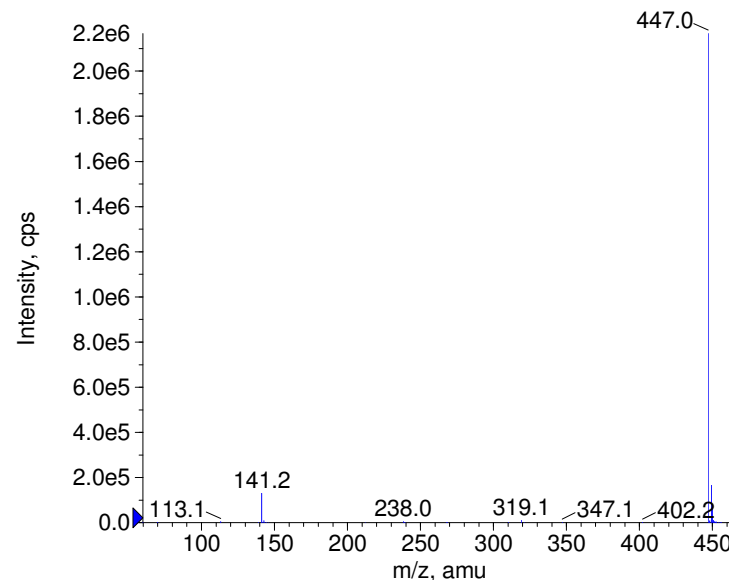
+ Thioproperazine Prec(447.0) CE(50.0) RT(0.9)
