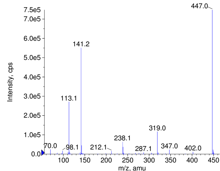
+ Thioproperazine Prec(447.0) CE(99.0) RT(0.9)
