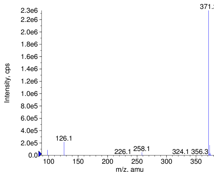
■ + Thioridazine Prec(371.0) CE(50.0) RT(0.7)
