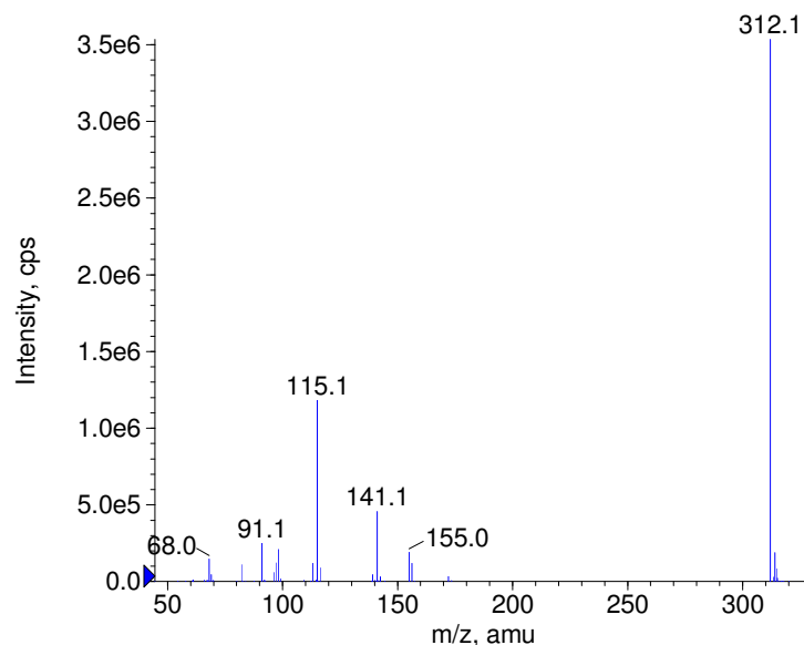
+ Tolazamide Prec(312.0) CE(50.0) RT(0.9)
