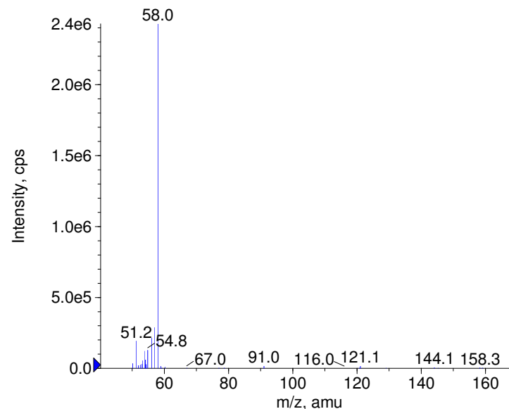
+ Tramadol Prec(264.0) CE(50.0) RT(0.7)
