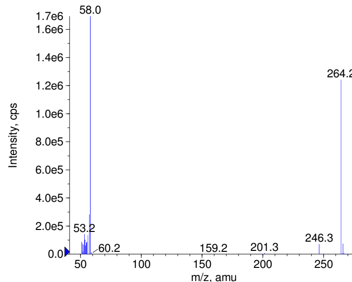
+ Tramadol Prec(264.0) CE(50.0) RT(0.7)
