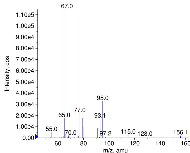
+ Tranexamic acid Prec(158.0) CE(50.0) RT(0.8)
