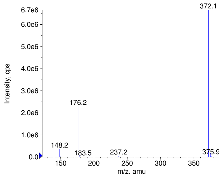
+ Trazodone Prec(372.0) CE(50.0) RT(0.7)
