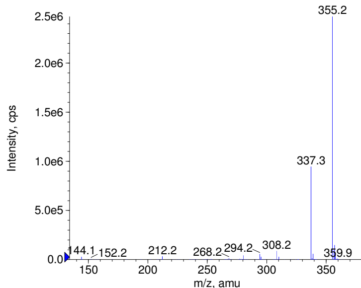
+ Vincamine Prec(355.0) CE(50.0) RT(0.7)
